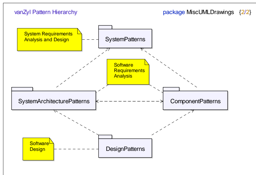
Figure 1 – van Zyl Pattern Hierarchy
